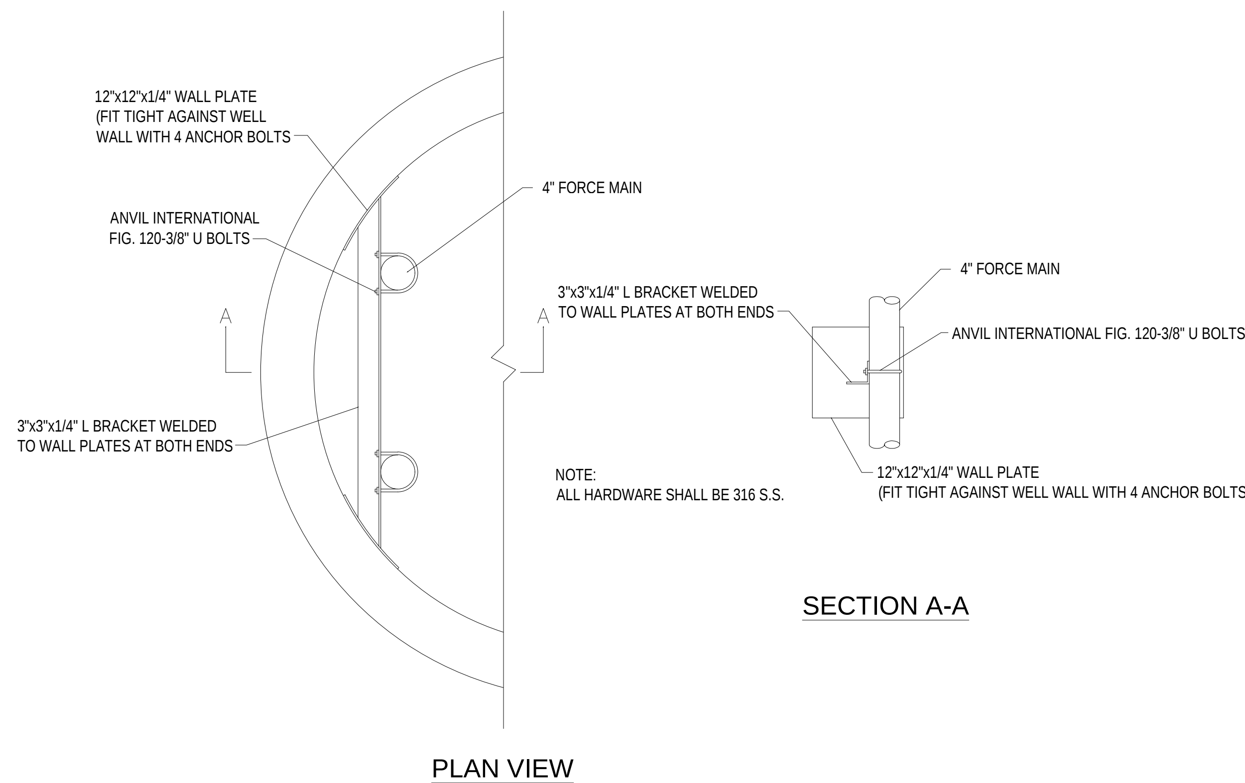
PLAN VIEW DISCHARGE PIPE SUPPORT DETAIL NOT TO SCALE
