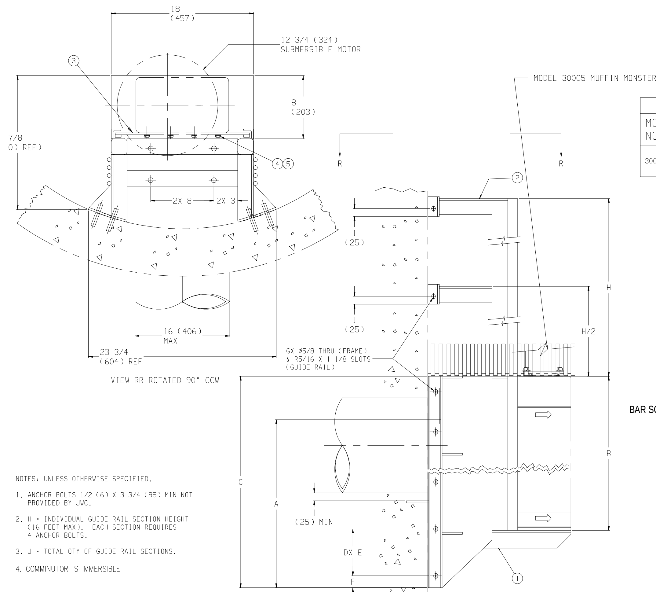
COMMUNOTOR MOUNTING DETAIL NOT TO SCALE
