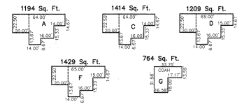
CONDOMINIUM UNIT TYPE DETAILING SCALE: 1" = 50'
